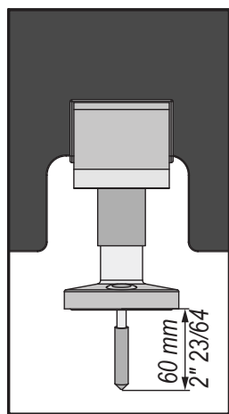
C. Leg of divider panel: fastening on the ground.
